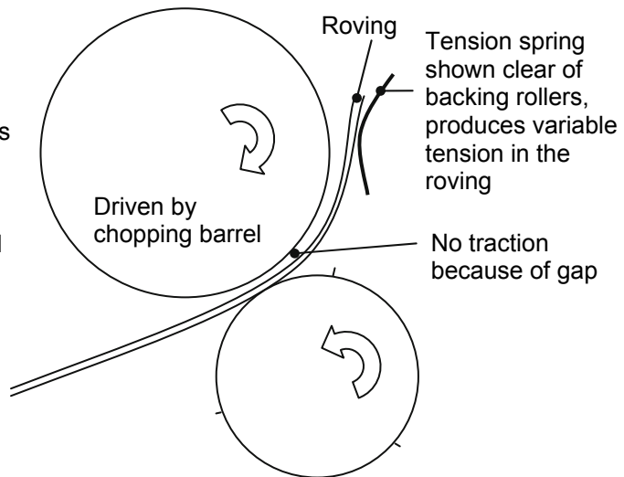
Backing Roller Spring Setting
