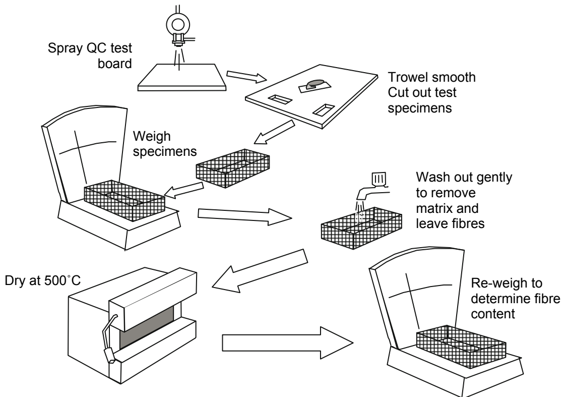
Procedure for determination of fibre content
