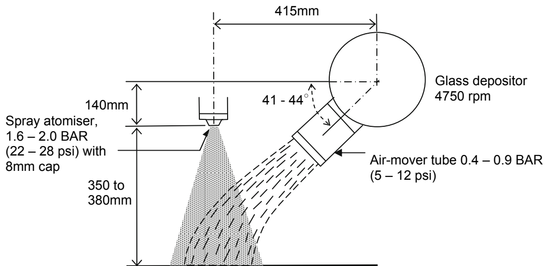
Arrangement of spray assembly with a single chopper
