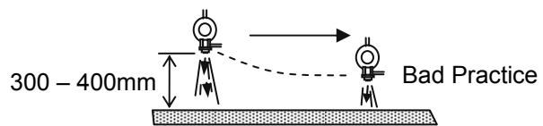
Always Spray Perpendicular to the Mould Surface and Maintain Constant Height
