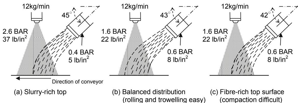
Illustration of Effect of Atomising Pressure and Angle of Deposition.
