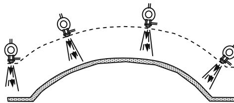
Always Spray Perpendicular to the Mould Surface and Maintain Constant Height
