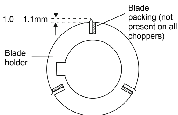
Blade Setting
